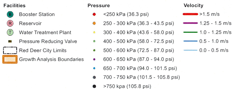
Figure 6.21: Scenario 5 Pressures and Pipe Velocities in the PHD - Current Standard City of Red Deer Water Model Update City of Red Deer
